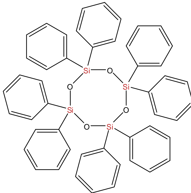
SiSiB ® PC9181 2,4,6,8-tetramethyl-2,4,6,8-tetraphenyl-cyclotetrasiloxane Synonym: Tetraphenyltetramethylcyclotetrasiloxane Tetramethyltetraphenylcyclotetrasiloxane
